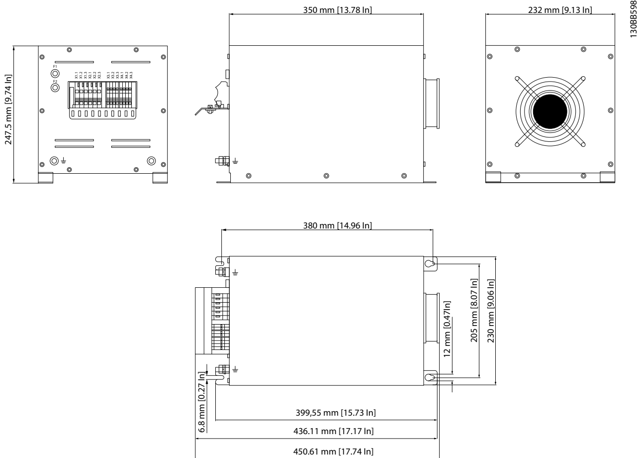
Illustration 6.4 X2 External Fan
