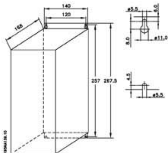
VLT 2855-2875 380-480V
