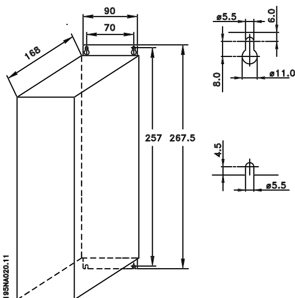
VLT 2822-2840 380-480V
