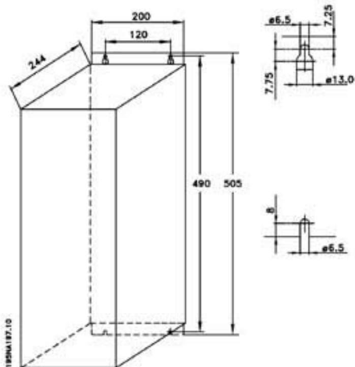
VLT 2880-82 380-480V
